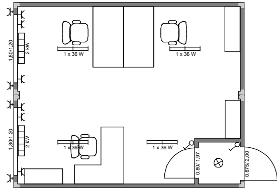
ARS DUO2 - 6,05m x 4,87m x RH 2,50m
