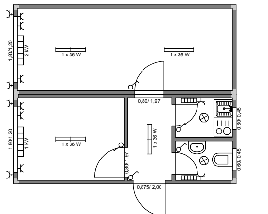
ARS DUO6 - 6,05m x 4,87m x RH 2,50m
