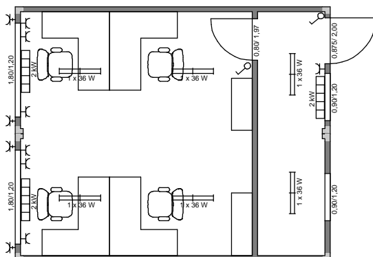
ARS DUO5 - 6,05m x 4,87m x RH 2,50m
