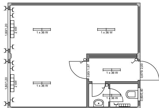
ARS DUO4 - 6,05m x 4,87m x RH 2,50m
