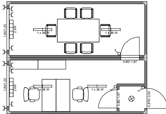
ARS DUO1 - 6,05m x 4,87m x RH 2,50m
