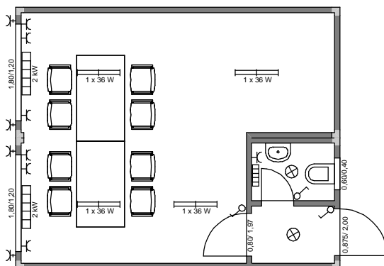
ARS DUO3 - 6,05m x 4,87m x RH 2,50m
