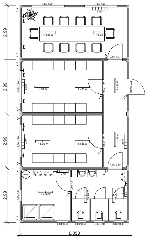
ARS V 6 - (LxB) 12,00m x 6,058m; RH = 2,50m
