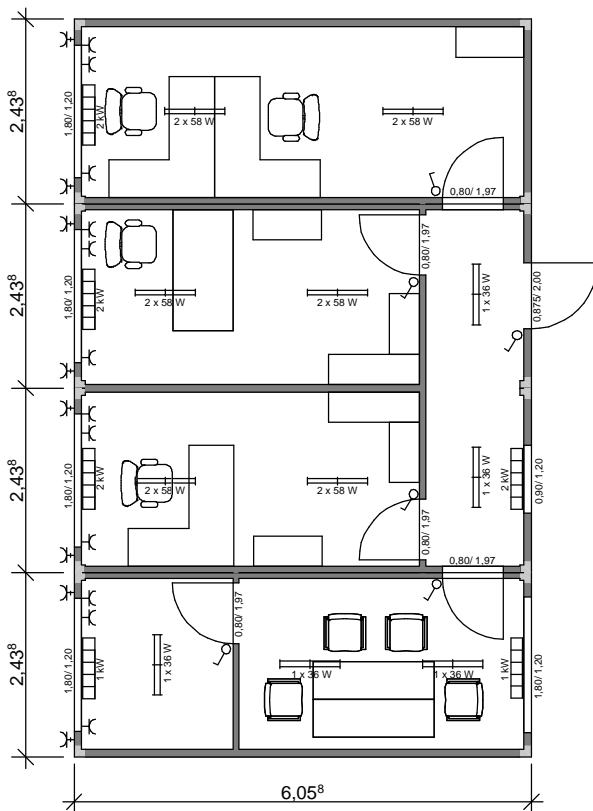
ARS V 5 - (LxB) 9,75m x 6,058m; RH = 2,50m
