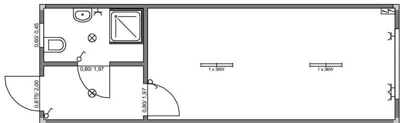
Typ D3S 04 - (LxB) 9,00m x 2,99m; RH = 2,50m
