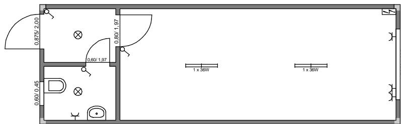
Typ D3S 03 - (LxB) 9,00m x 2,99m; RH = 2,50m
