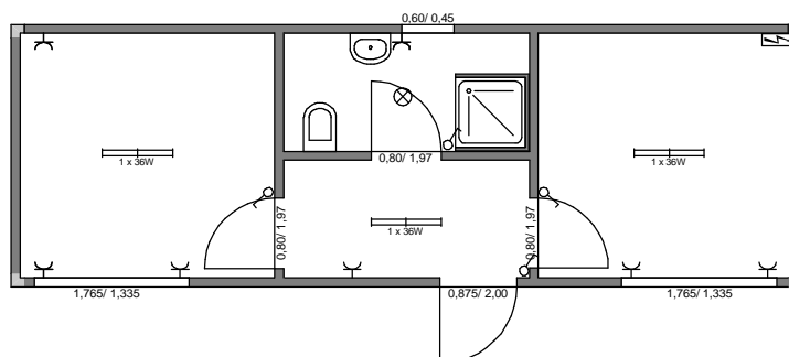
Typ D3S 08 - (LxB) 9,00m x 2,99m; RH = 2,50m
